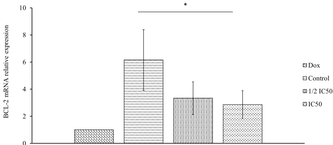
Figure 1. mRNA relative expression of BCL-2 in each group. Control : Untreated MDA-MB-231 cells , \frac{1}{2} IC_{50} : CSCs treated with trisindoline 5 in \frac{1}{2} IC_{50} dose, IC_{50} : CSCs treated with trisindoline 5 in IC_{50} dose, and Dox : CSCs treated with doxorubicin. * Indicates a significant difference from the control group ( P < 0.05 ); indicates a significant difference from the control ( P < 0.05 ; n = 3 per group). The data represent mean \pm standard deviation (SD).
